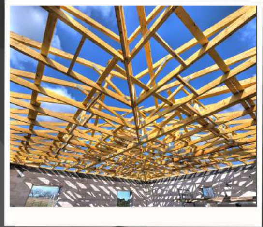
Roofing Timber
